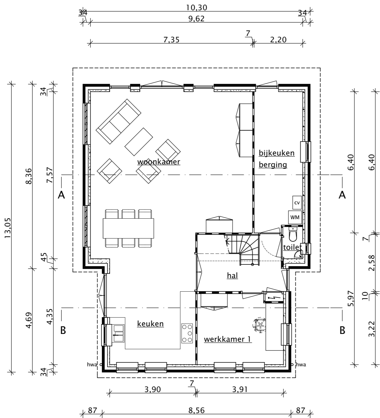
plattegrond BEGANEGROUND
